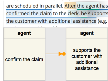
Fig. 2: Correspondence between text and DCR graphs
